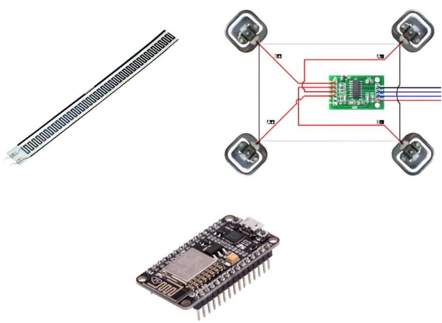
ESP32 receives data from FSR & Load Cell sensors
